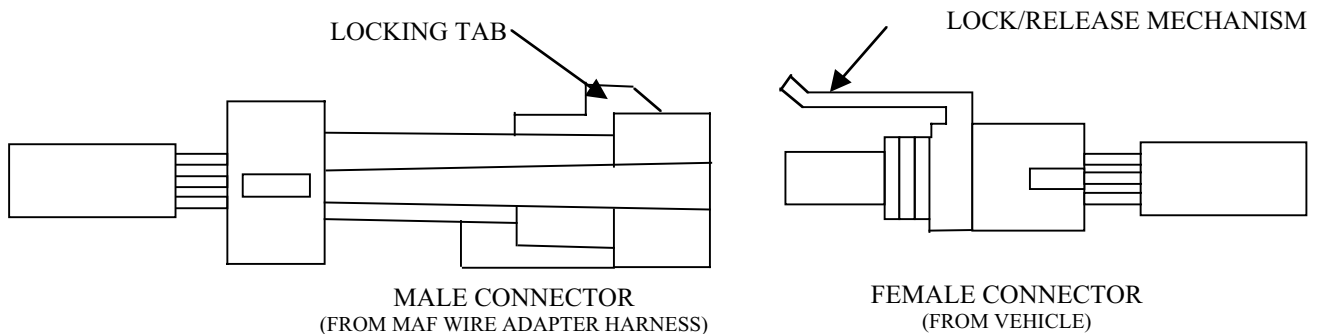
Figure 1: MAF wire adapter harness connection (side view).
